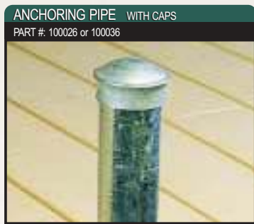
Galvanized steel, mechanical-grade pipe provides economical anchoring in shallow water. Pipe and caps sold separately.
